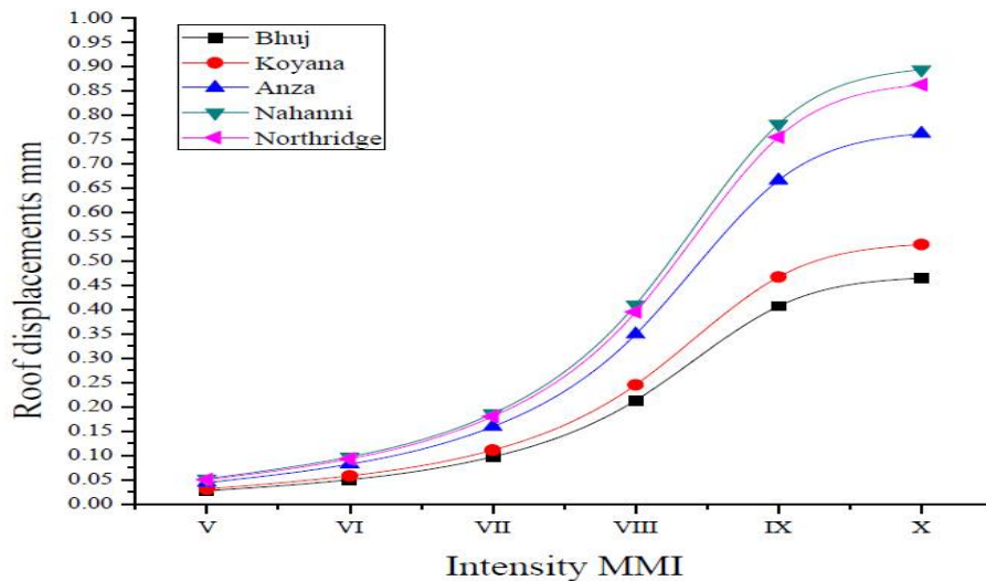
Figure 4: Variations in Roof Displacements for X Directions
