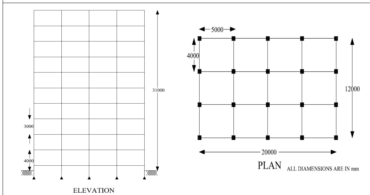
Figure 1: Plan and Elevation of Multistoried Building
