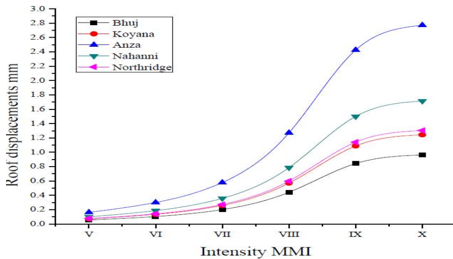
Figure 5: Variations in Roof Displacements for X Directions
