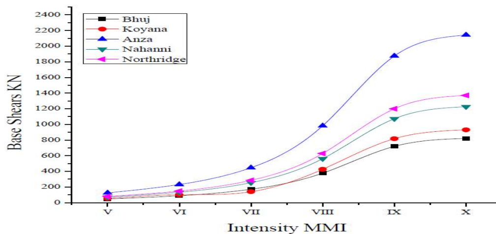
Figure 3: Variations in Base Shears for Y Directions
