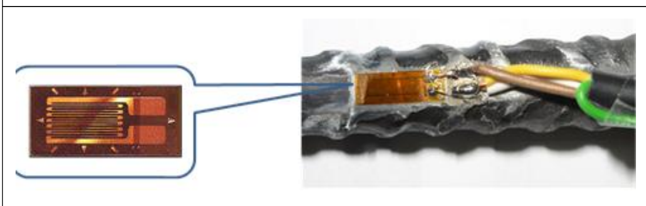
Figure 3: Detail of bonded and welding of electric gauge
