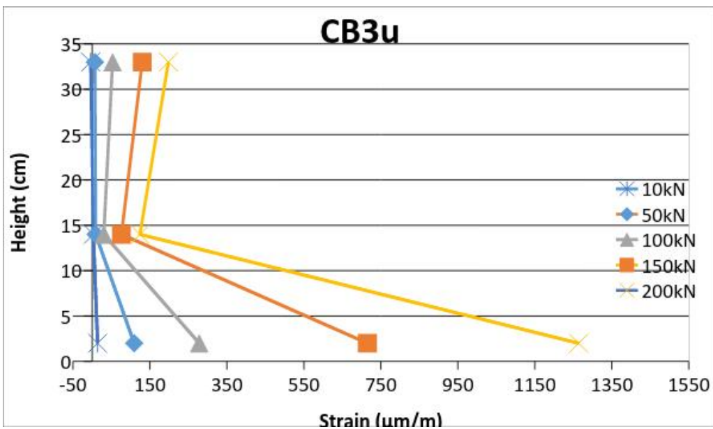
Figure 7: Position of Neutral Axial Versus Applied Load for CB3u
