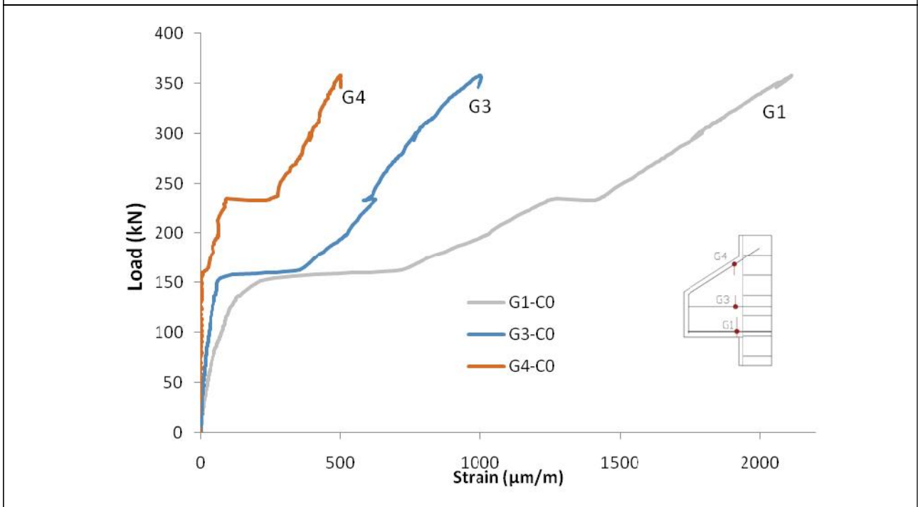
Figure 4: Local Strain of Steel in Cross Section of Reinforced Concrete Corbel
