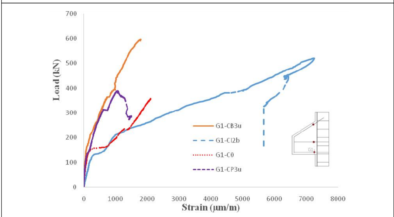
Figure 5: Comparison of Steel Strain in Cross Section (point G1) of Strengthened Corbel
