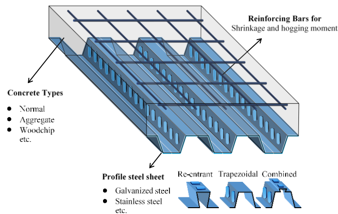
Figure 1. Typical composite slab
